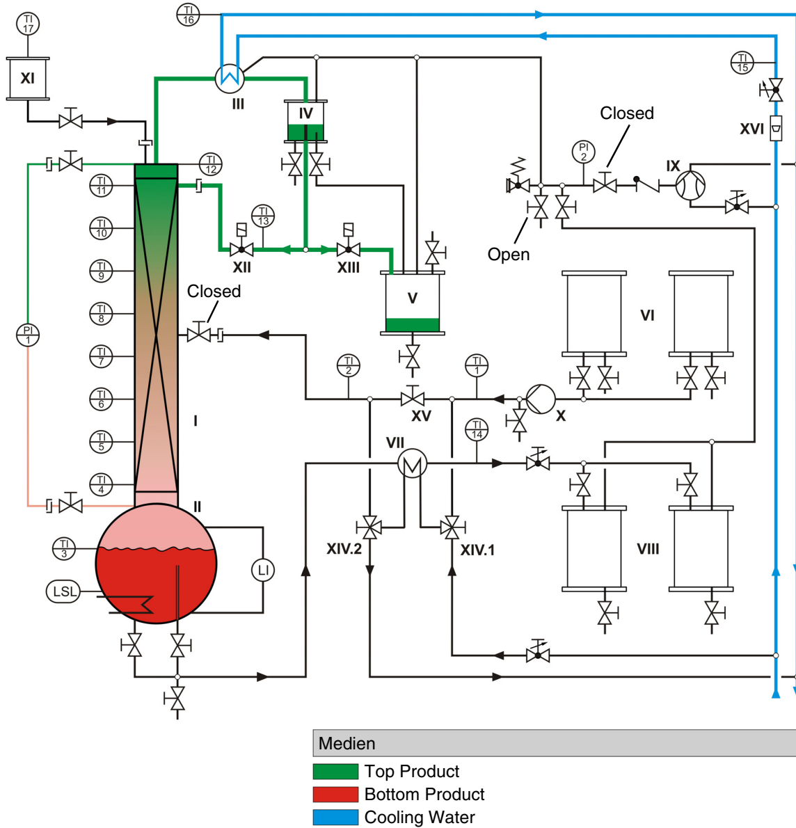
Fig. 5.10 Process diagram for a batch experiment at ambient pressure
